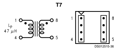
Top View FIGURE 21. Pulse PE-68482
