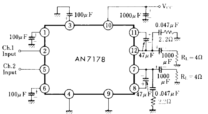
Test Circuit 1
