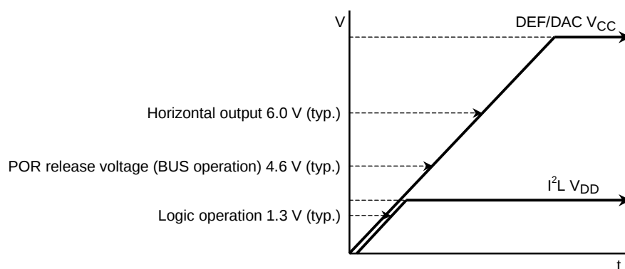
Figure B Timing chart that indicates the timing from power-on till horizontal output. (At Ta = 25 C°)
