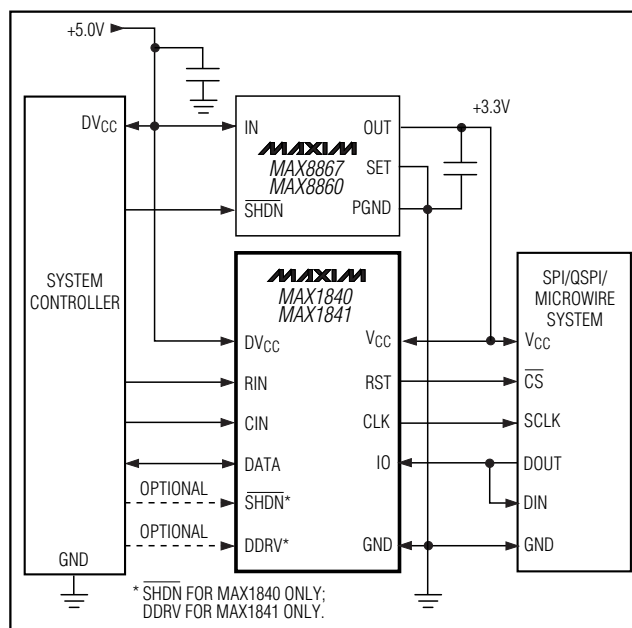
Figure 3. MAX1840/MAX1841 with SPI/QSPI/MICROWIRE Interfaces
