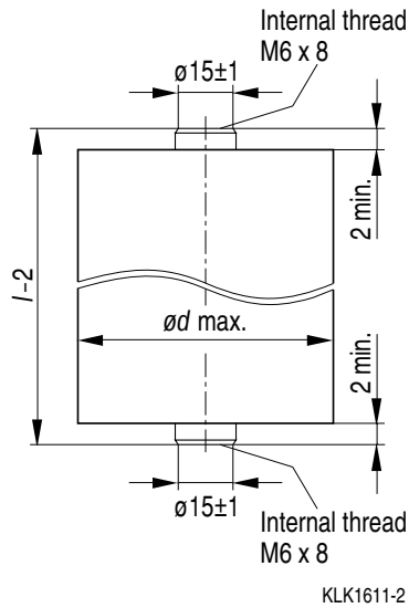
Dimensional drawing 1
