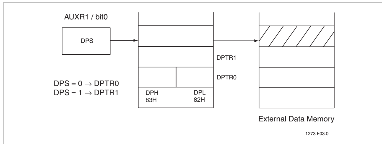
FIGURE 3-3: Dual Data Pointer Organization
