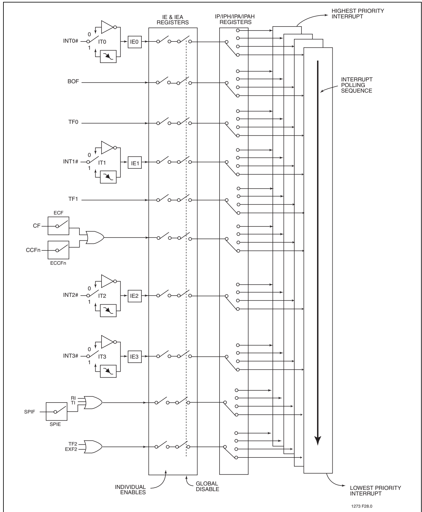
FIGURE 11-1: Interrupt Structure
