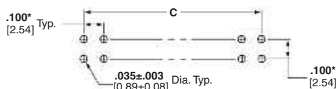
Recommended PC Board Hole Layout (for .055 [1.40] min. thick PC board)
