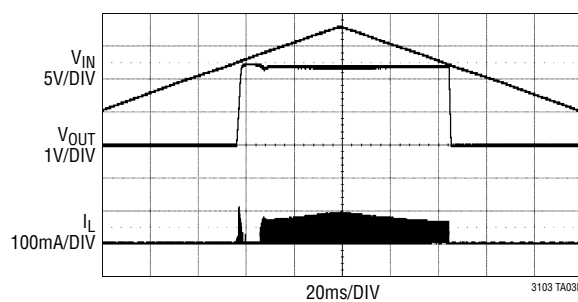
Start-Up with Ramped Input Power
