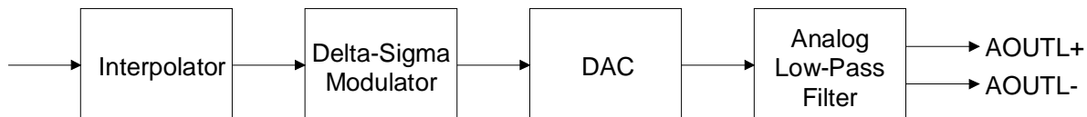
Figure 2. Block Diagram
