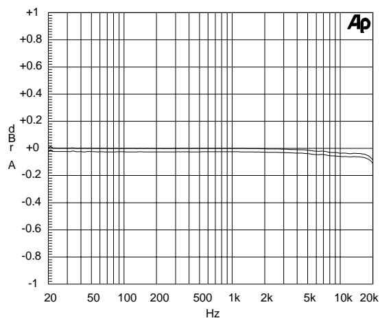
Figure 14. Frequency Response
