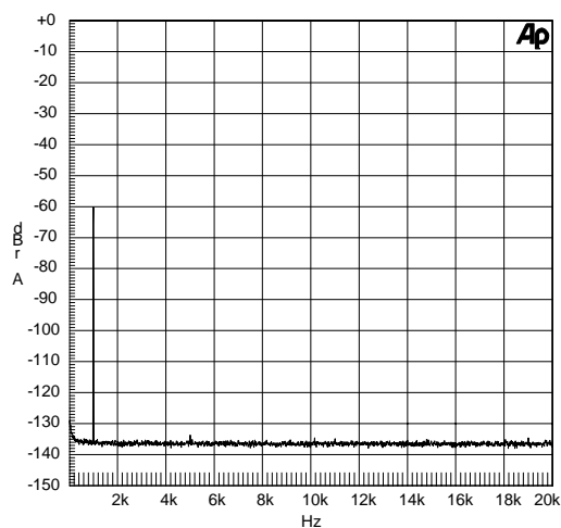
Figure 18. -60 dBFS FFT
