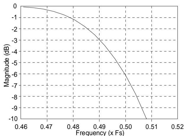
Figure 11. Combined Digital and Analog Filter
