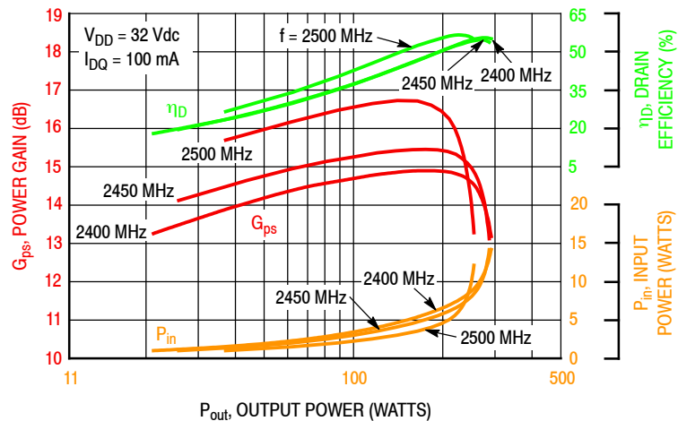
Figure 6. Power Gain, Drain Efficiency and Input Power versus Output Power and Frequency
