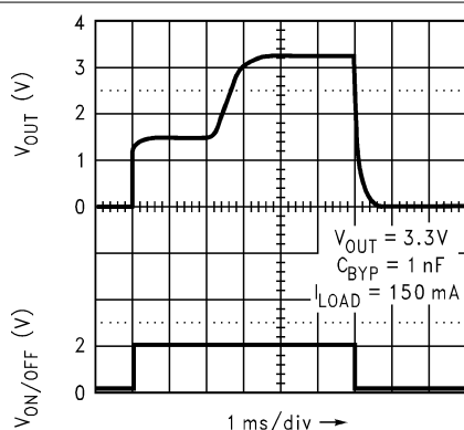
Figure 7-24. Turn-On Time (Legacy Chip)
