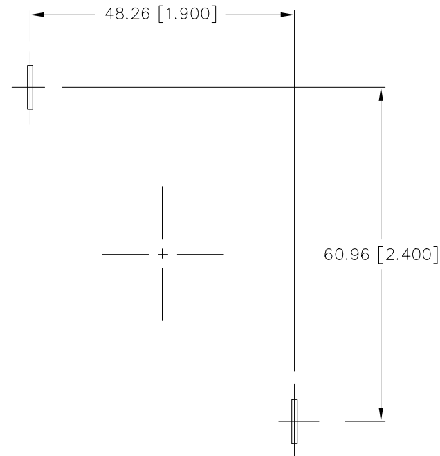
REF: ANCHOR LAYOUT
