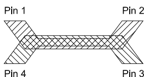
Directional Coupler Pin Configuration
