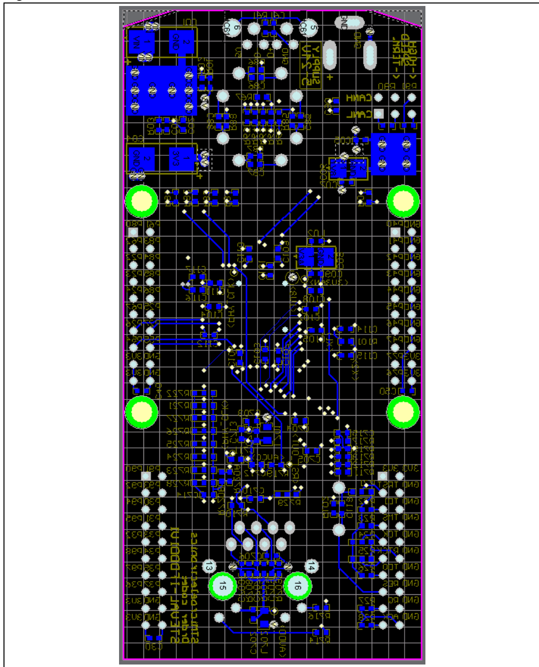
Figure 8. Bottom view
