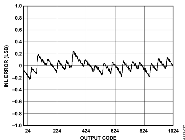
Figure 17. AD9204-80 INL with f_{IN} = 9.7\text{ MHz}
