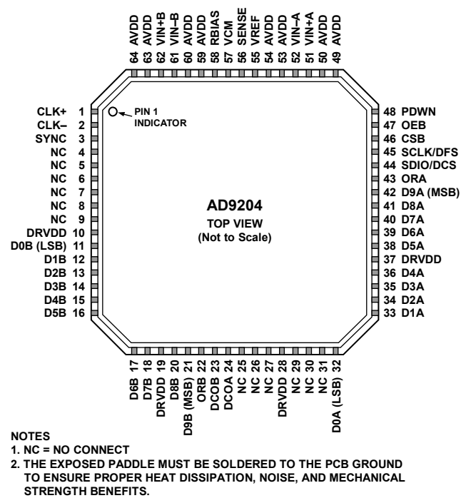
Figure 5. Pin Configuration
