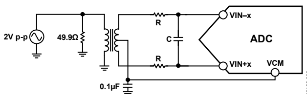
Figure 42. Differential Transformer-Coupled Configuration
