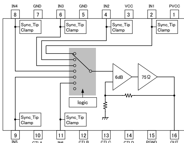
Fig.1 BH76360FV
