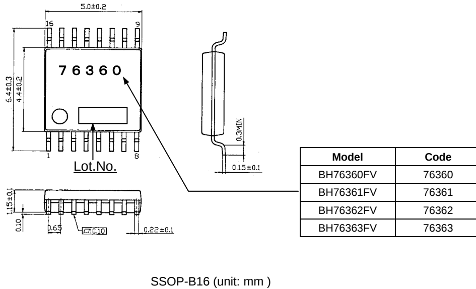
Fig.101 External Dimensions of BH7636xFV Series Package
