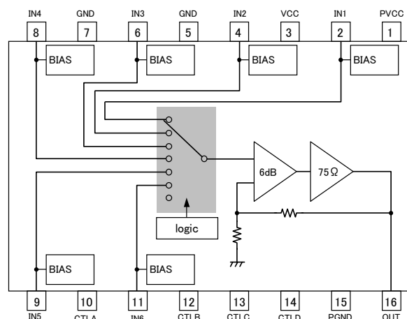
Fig.2 BH76361FV
