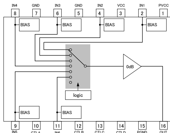
Fig.4 BH76363FV
