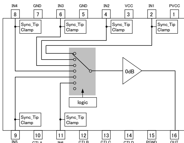
Fig.3 BH76362FV
