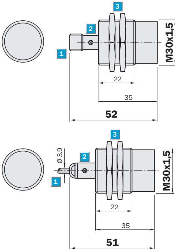
Dimensional drawing
