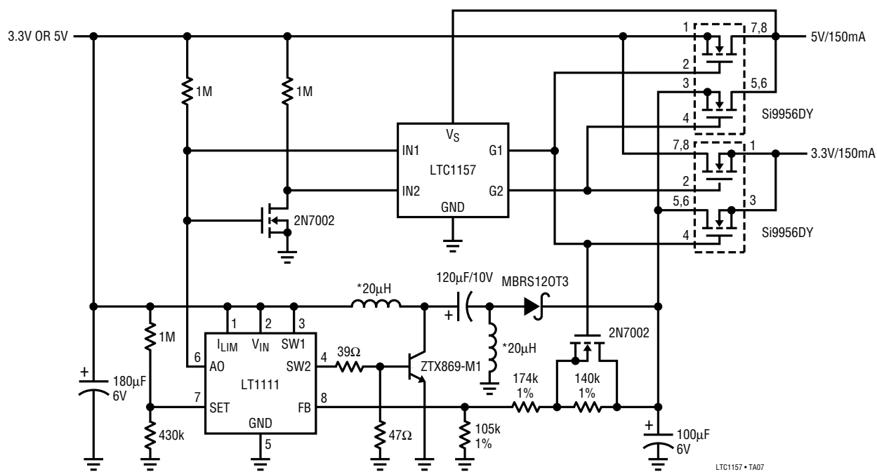
Generating 3.3V and 5V from a 3.3V or 5V Source (Automatic Switching)
