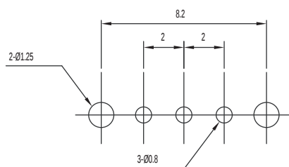
PIERCING PLAN
