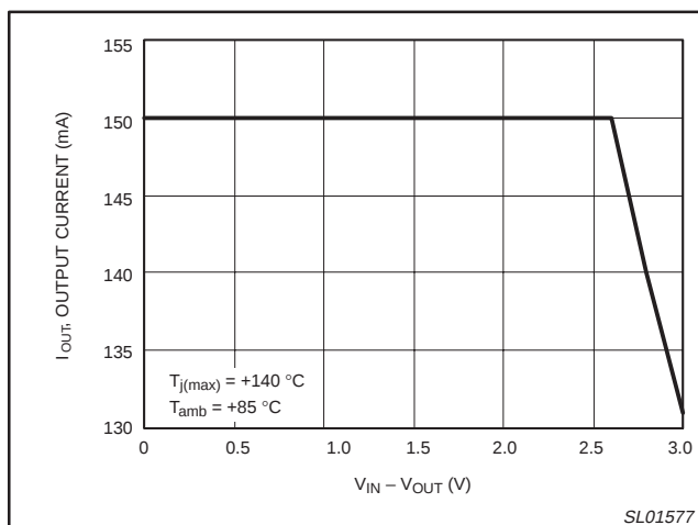
Figure 8. Maximum I_{OUT} versus V_{IN} - V_{OUT} .
