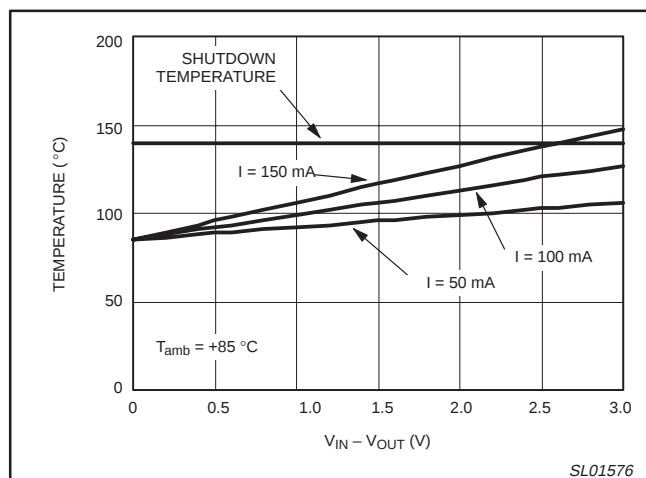
Figure 7. T_j versus V_{IN} - V_{OUT} for 3 output currents.
