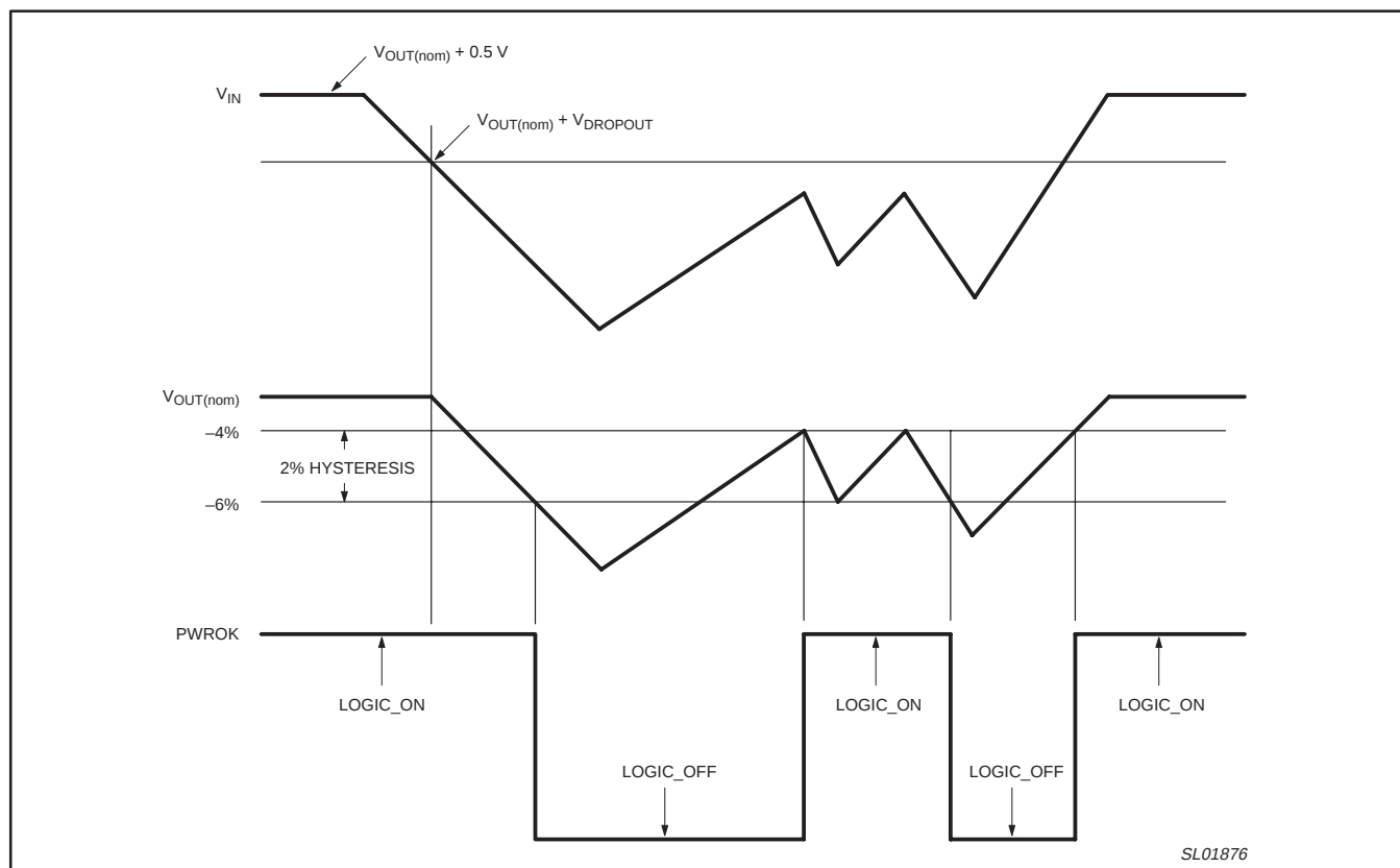
Figure 13. Timing diagram.
