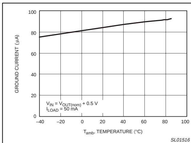
Figure 4. Ground current versus temperature.
