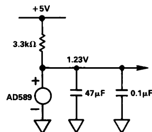
Figure 14. Reference Circuit
