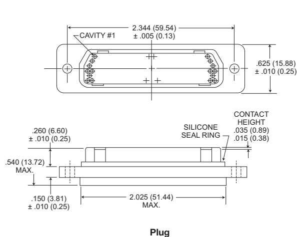
Plug
