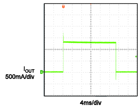
Current Limit
