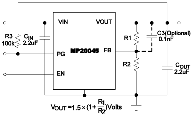
Adjustable Version
