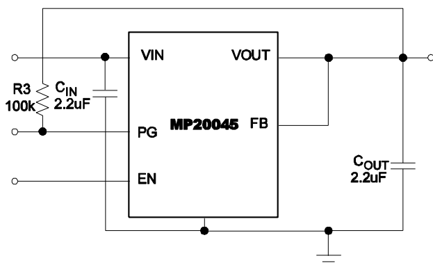
Fixed Version
