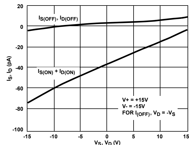
FIGURE 18. LEAKAGE CURRENT vs ANALOG VOLTAGE
