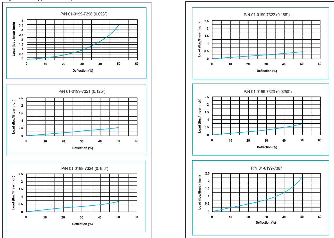
Figure 1 - Typical Compression/Deflection
