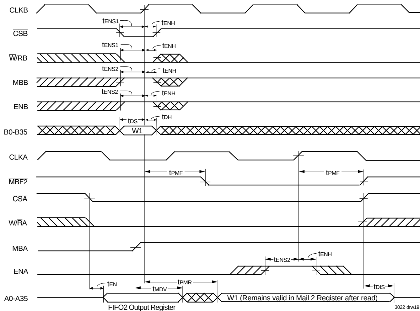
Figure 17. Timing for Mail2 Register and \overline{MBF2} Flag
