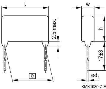
Straight leads
