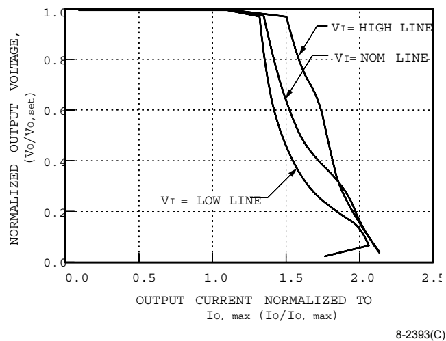
Figure 4. Lx005x Normalized Output Current vs. Normalized Output Voltage at T_c = 25^\circ\text{C}
