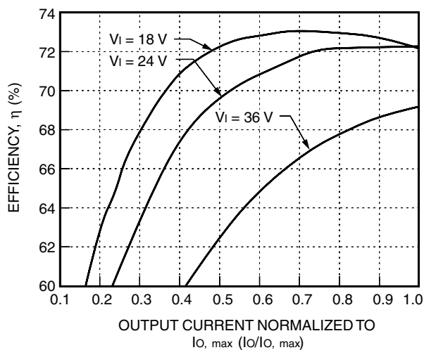
Figure 5. LC005F Typical Efficiency vs. Normalized Output Current at T_c = 25\text{ }^{\circ}\text{C}
