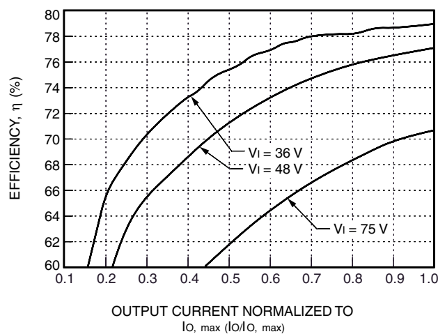
Figure 10. LW005B Typical Efficiency vs. Normalized Output Current at T_c = 25^\circ\text{C}
