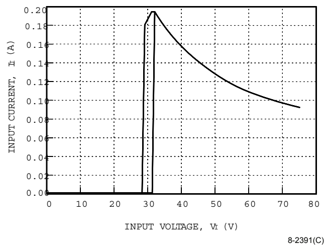
Figure 2. LW005x Input Current vs. Input Voltage at I_o = I_{o, \max} and T_c = 25^\circ\text{C}
