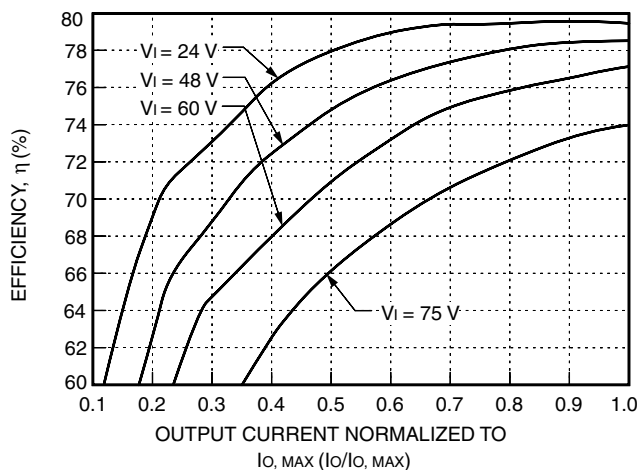
Figure 9. LW005A Typical Efficiency vs. Normalized Output Current at T_c = 25^\circ\text{C}
