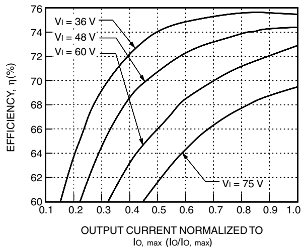
Figure 8. LW005F Typical Efficiency vs. Normalized Output Current at T_c = 25\text{ }^{\circ}\text{C}
