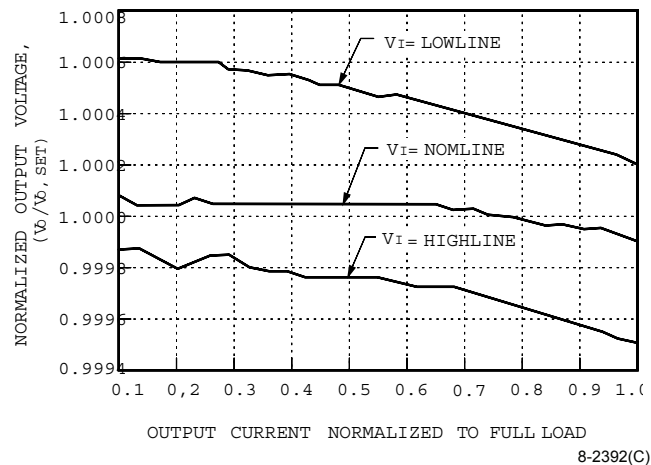
Figure 3. LW005x Load Regulation, Normalized Output Voltage vs. Normalized Output Current at T_c = 25^\circ\text{C}
