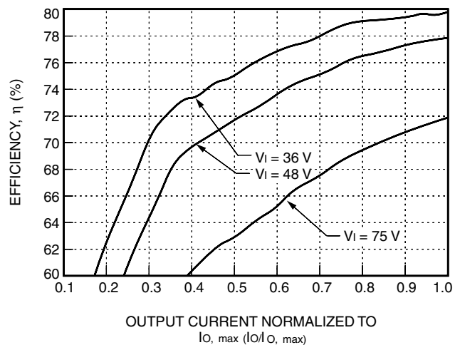
Figure 11. LW005C Typical Efficiency vs. Normalized Output Current at T_c = 25^\circ\text{C}
