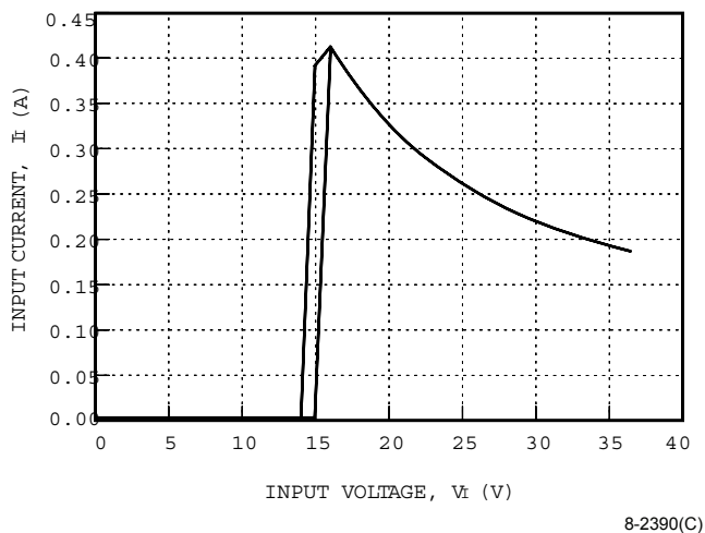
Figure 1. LC005x Input Current vs. Input Voltage at I_o = I_{o, \max} and T_c = 25^\circ\text{C}
