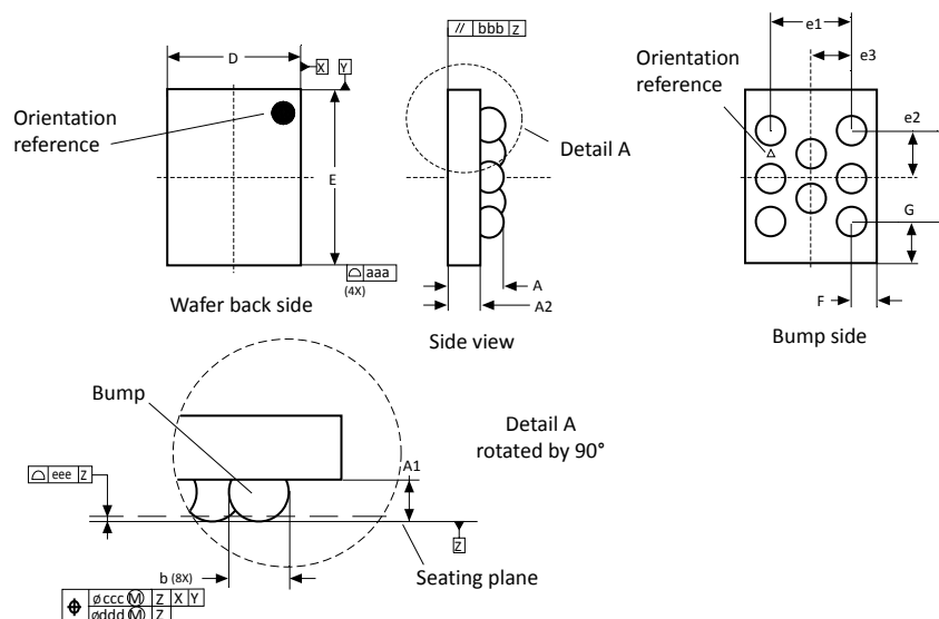
Figure 29. WLCSP8 - Outline
