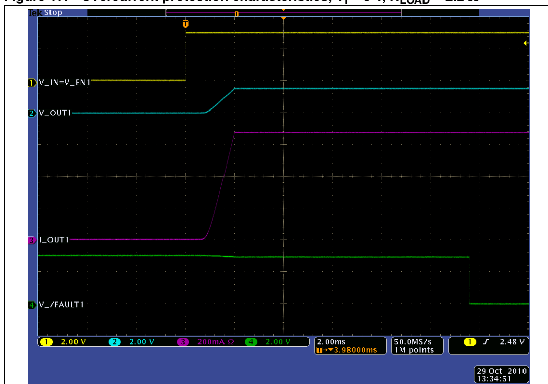
Figure 17. Overcurrent protection characteristics, V_I = 3\text{ V} , R_{\text{LOAD}} = 2.2\ \Omega
