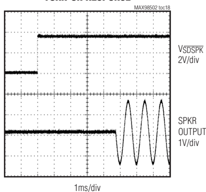
TURN-ON RESPONSE
