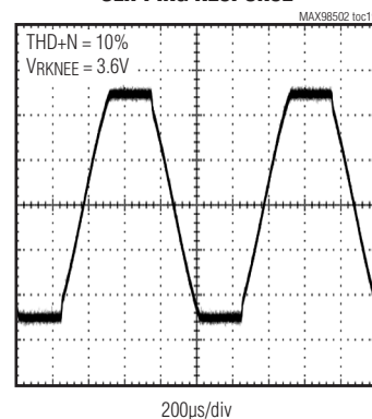
CLIPPING RESPONSE
