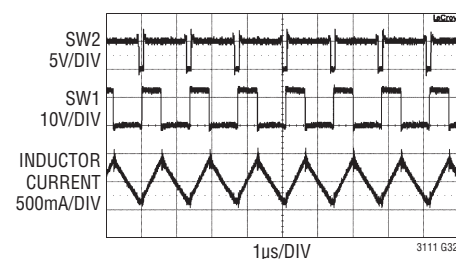
12V IN to 5V OUT SW1 and SW2 Waveforms
