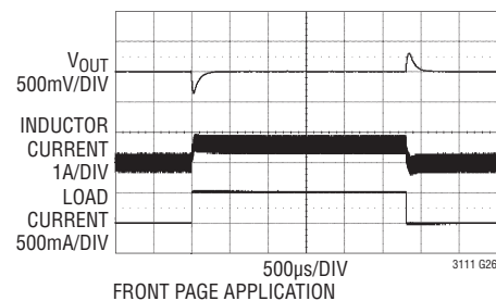
12V IN to 5V OUT 0.05A to 0.5A Load Response
