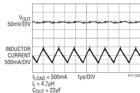
12V IN to 5V OUT PWM V OUT Ripple
