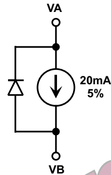
Equivalent Block Diagram
