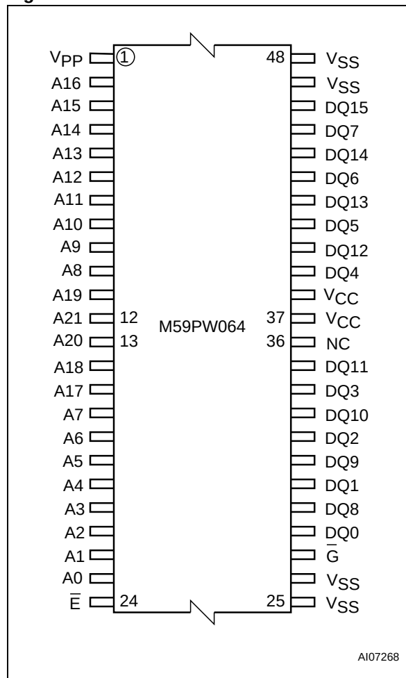
Figure 4. TSOP Connections
