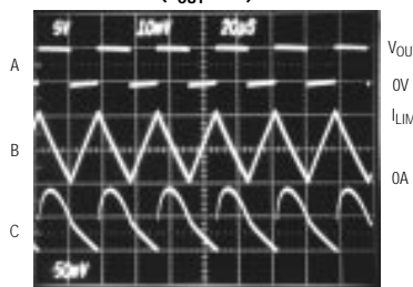
MEDIUM-LOAD SWITCHING WAVEFORMS ( V_{OUT} = 5V )
