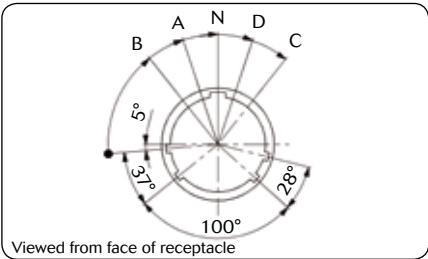
Viewed from face of receptacle
