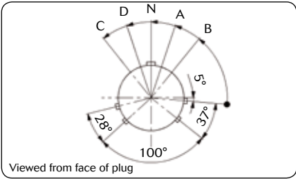
Viewed from face of plug
