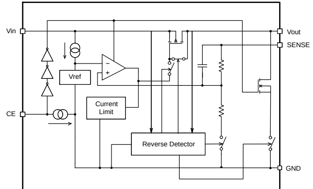
Figure 41. Reverse Operating Mode
