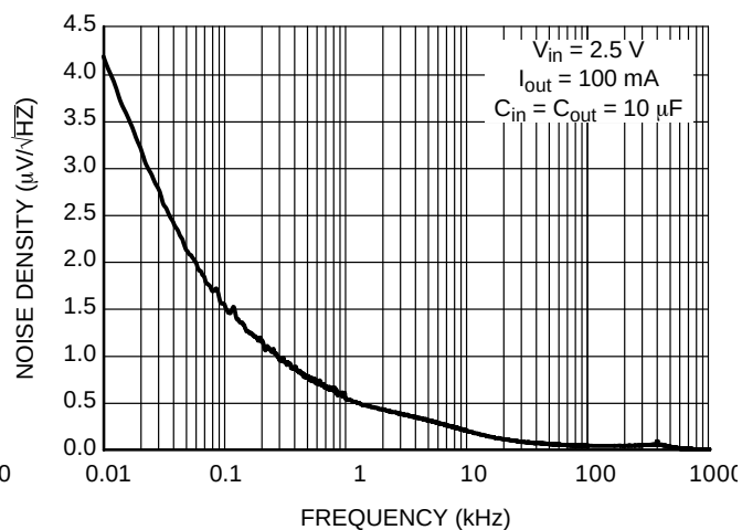
Figure 22. Output Noise Density vs. Frequency at NCP4632xDT15
