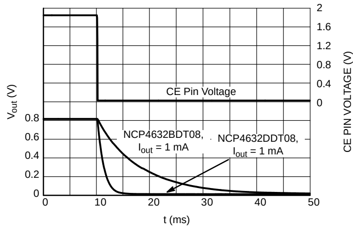
Figure 33. Turn Off with CE pin at NCP4632BDT08, NCP4632DDT08, I_{out} = 1 mA
