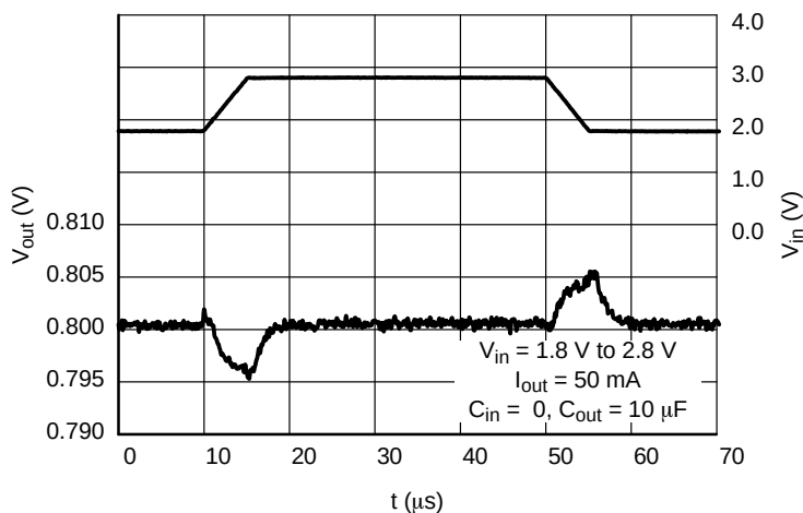
Figure 25. Line Transient Response at NCP4632xDT08
