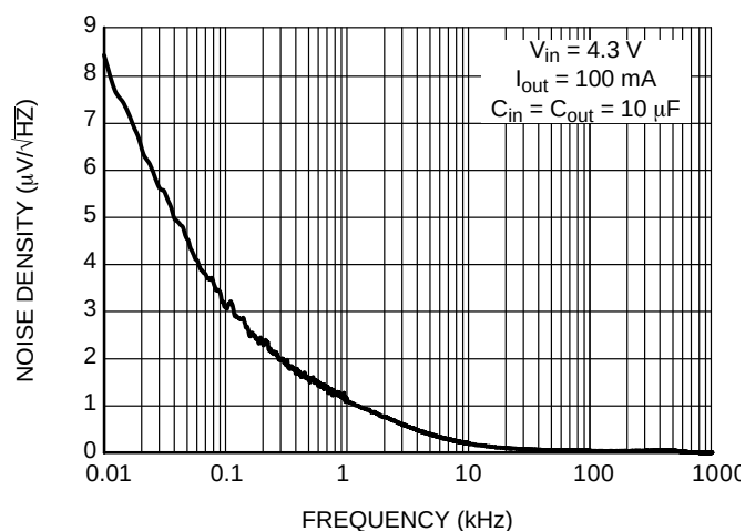
Figure 24. Output Noise Density vs. Frequency at NCP4632xDT33
