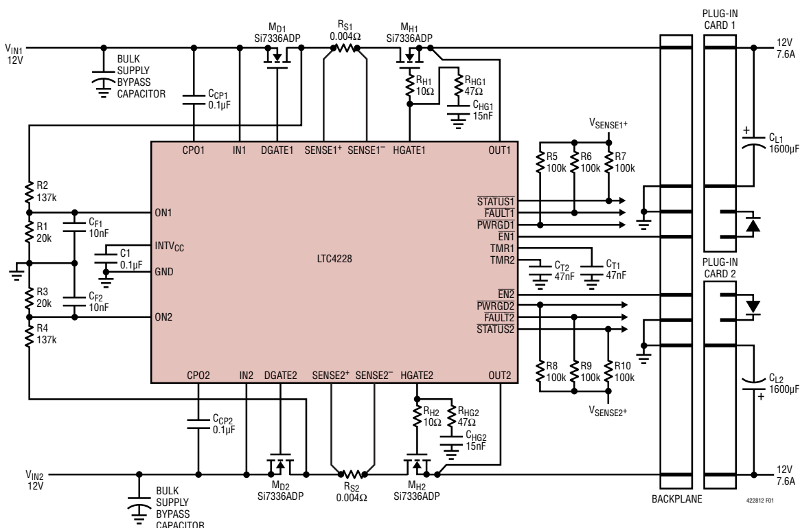
Figure 1. \mu TCA Application Supplying 12V Power to Two \mu TCA Slots
