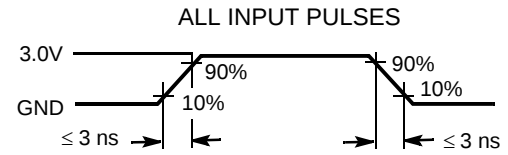
Figure 5. AC Test Loads and Waveforms [13, 14]
