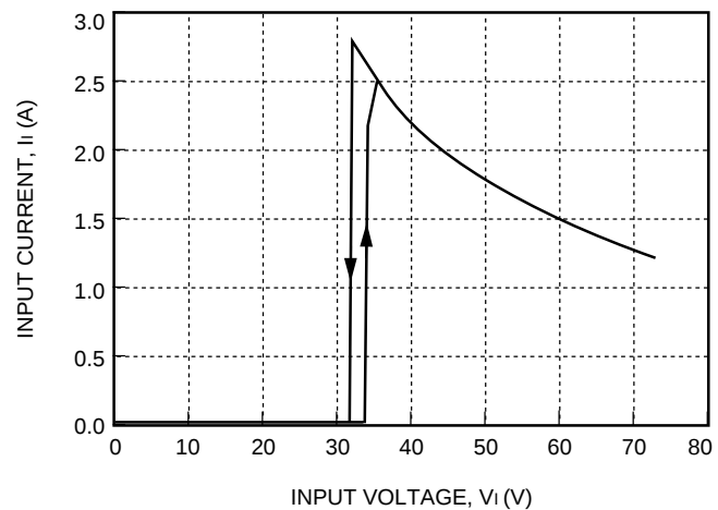
Figure 2. Typical JW075B Input Characteristics at Room Temperature
