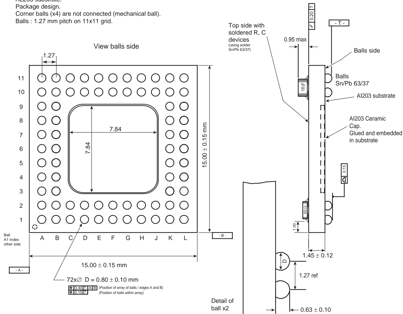
Figure 54. Package Dimension – 68 Pins CBGA
