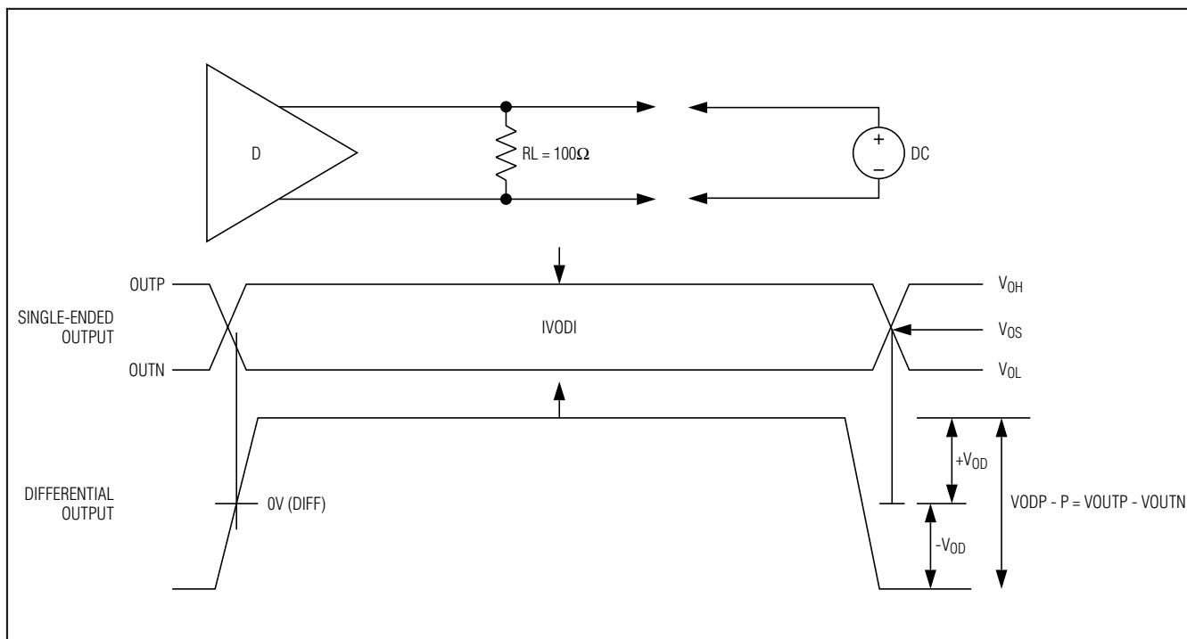
Figure 2. LVDS Level Definitions
