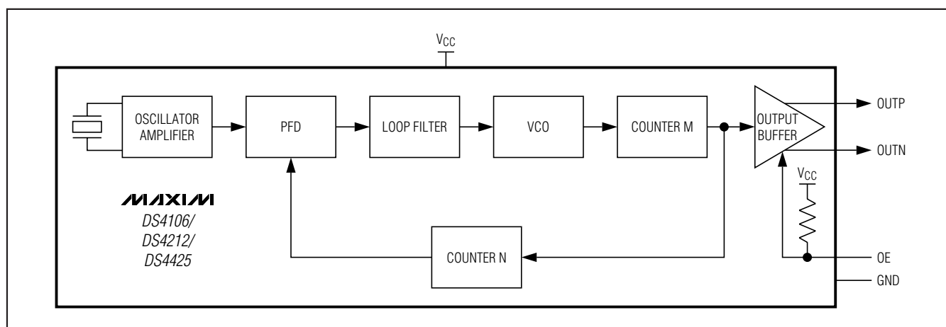
Figure 1. Functional Diagram
