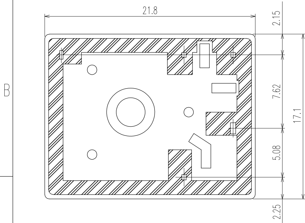
GENERAL TOLERANCE
