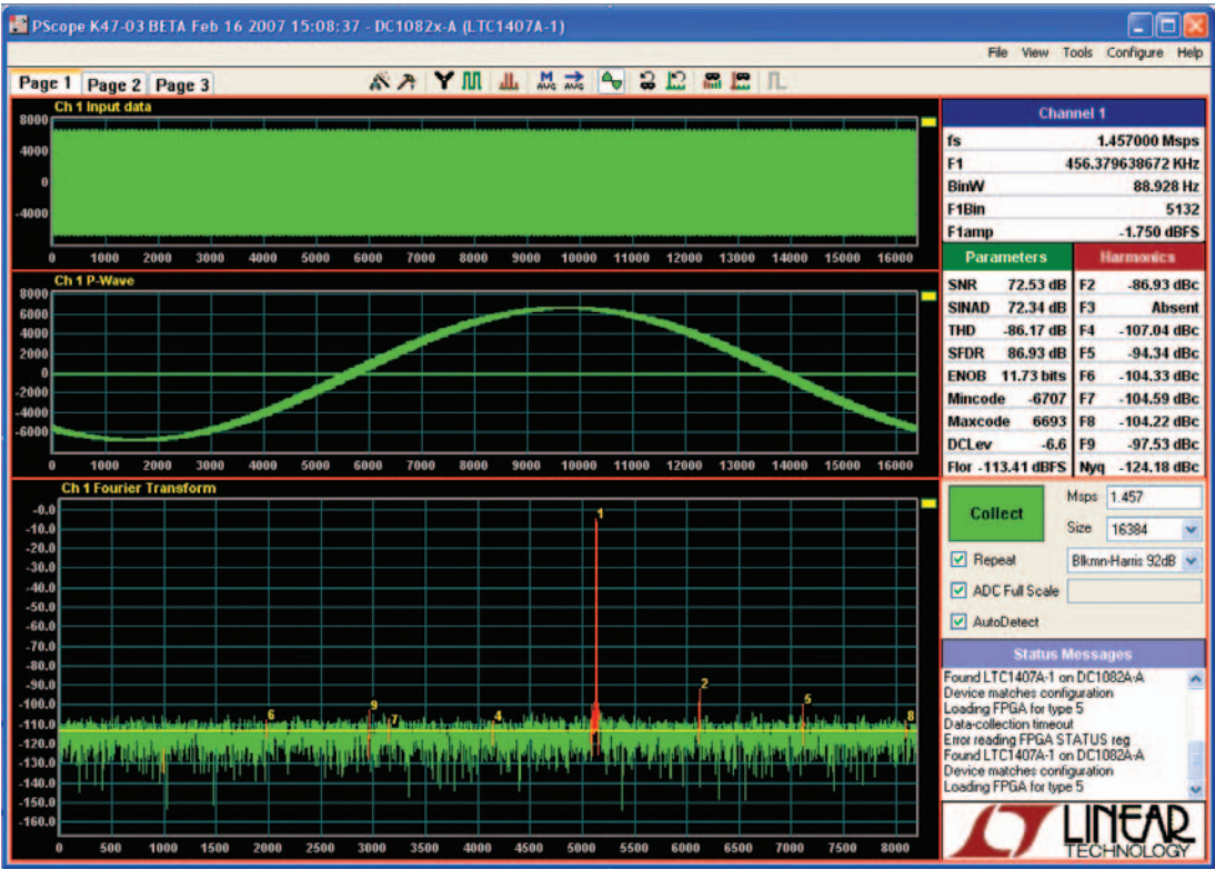
Figure 2. DC1082A Screenshot
