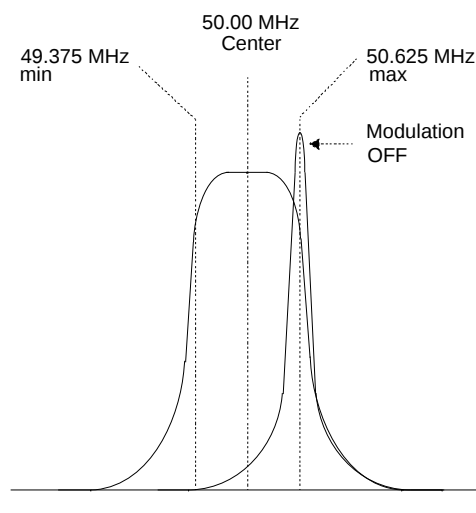
Figure 5. Output Clock
