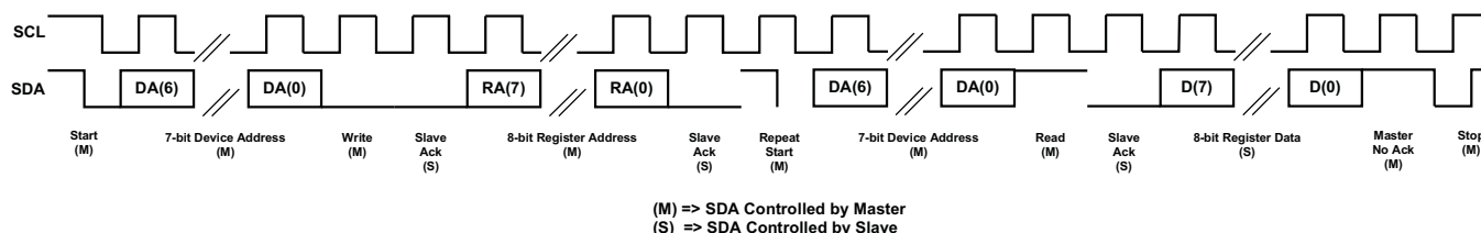
Figure 36. I²C Read
