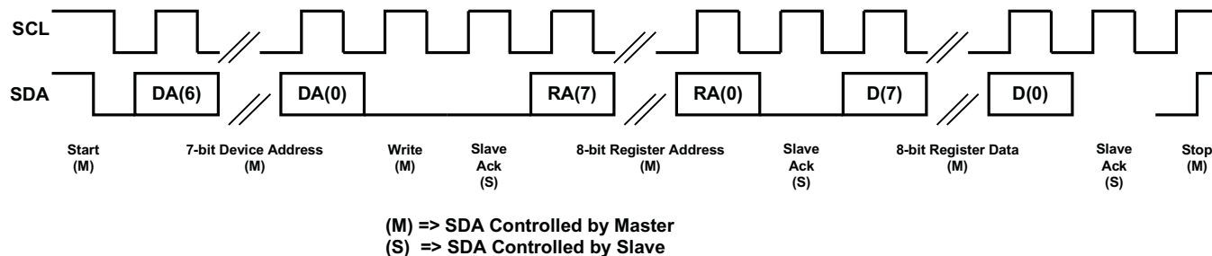
Figure 35. I²C Write
