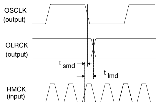
Figure 1. Audio Port Master Mode Timing
