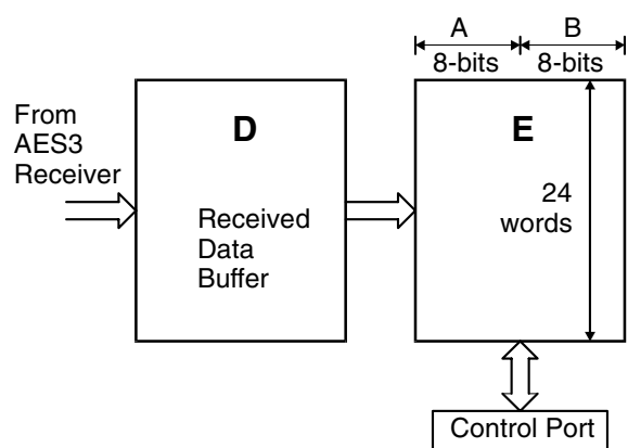
Figure 17. Channel Status Data Buffer Structure
