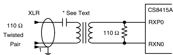
Figure 12. Professional Input Circuit
