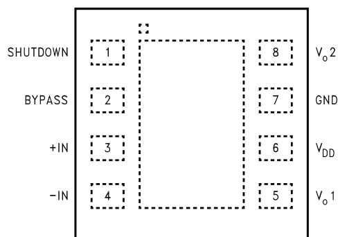
WSOP Package (Top View) Package Number NGL
