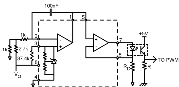
Optocoupler Driver Circuit for Power Supply Isolation
