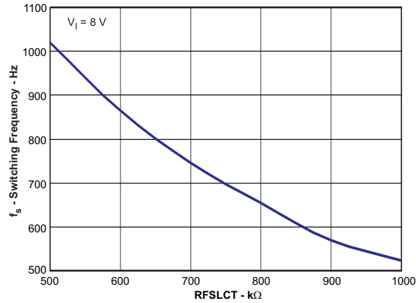
Figure 3. Switching Frequency
